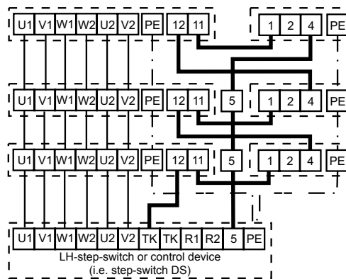
LH-unit with thermal cutouts and anti-frost thermostat
