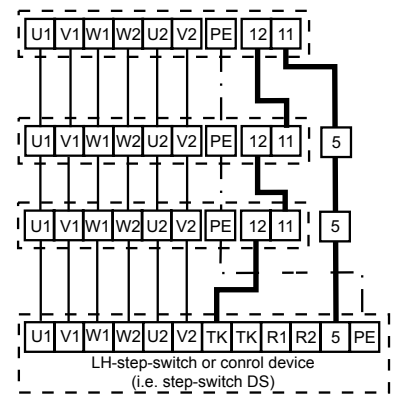
LH-unit with thermal cutouts
